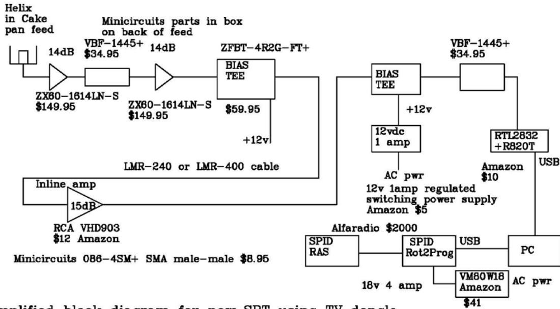
Simplified block diagram for new SRT using TV dongle
